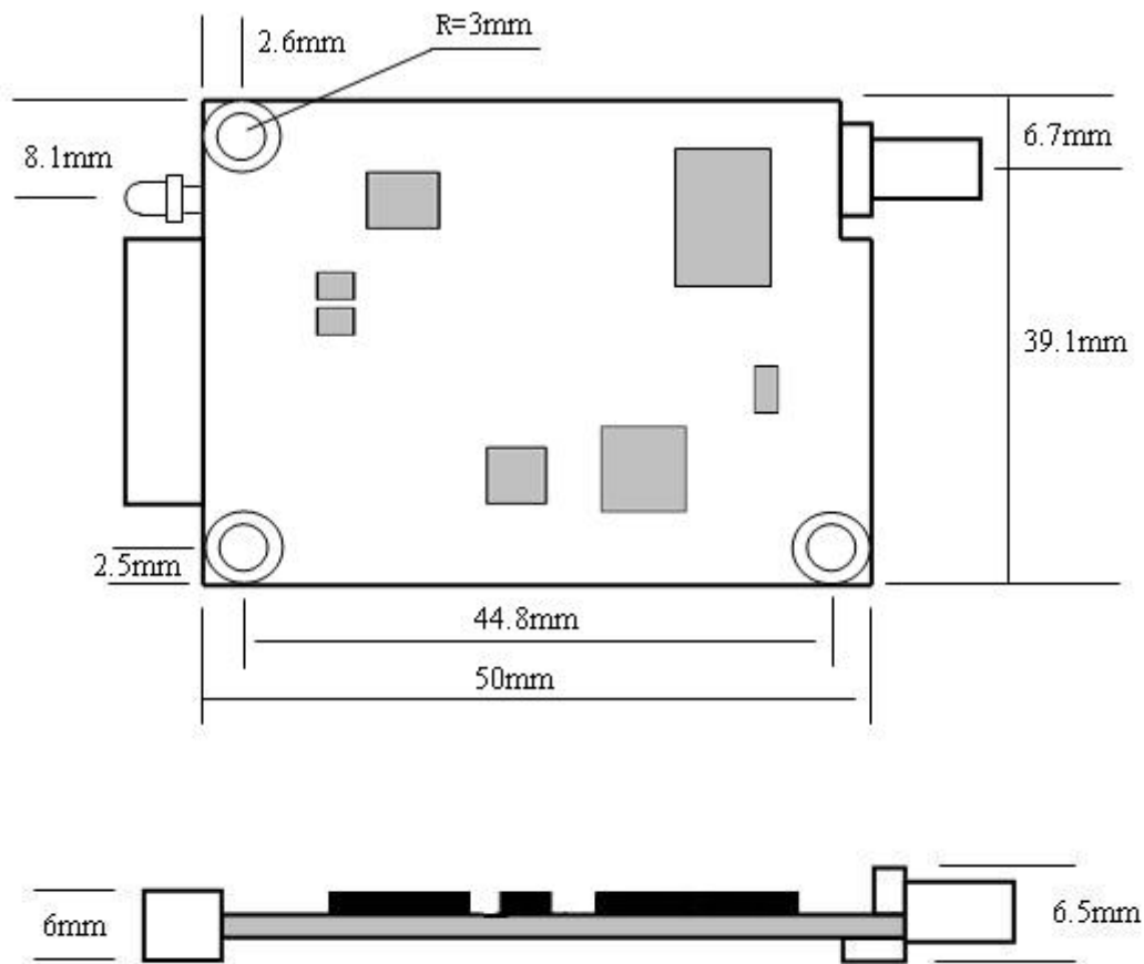
Figure 5: Mechanical Dimension
