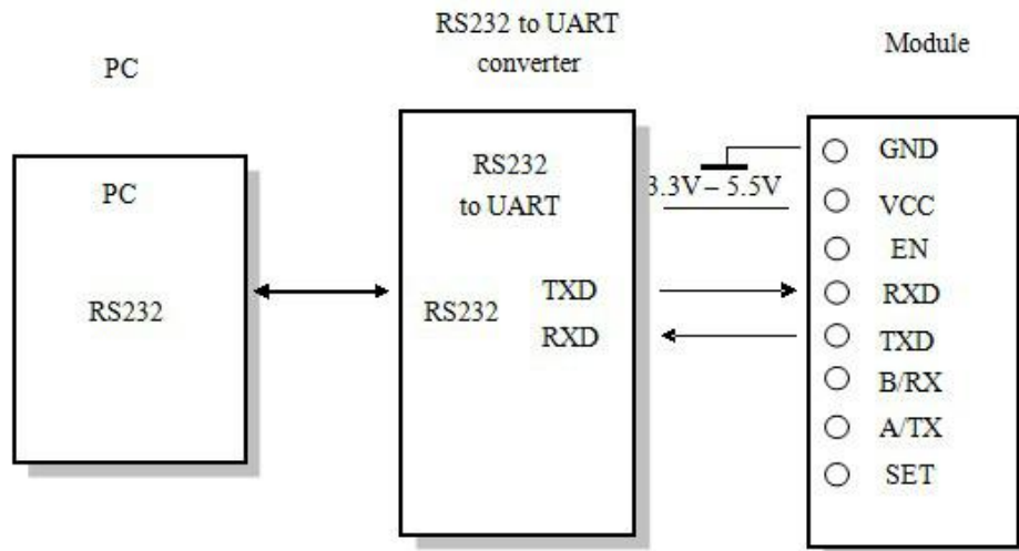
Figure 2: Connection Diagram
